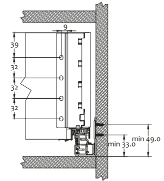
Mounting dimensions Back panel
