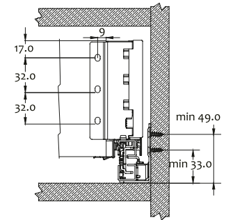
Mounting dimensions Back panel
