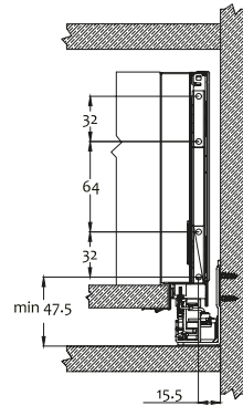
Mounting dimensions Front brackets
