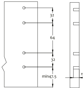
Drilling dimensions Front panel
