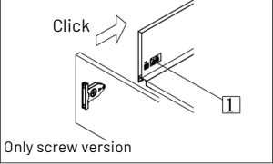
Left & right (side) adjustment :±1mm
