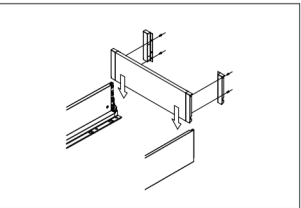
Drawer installation
