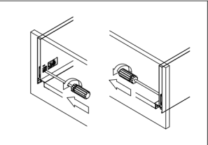
Left & right (side) adjustment :±1mm
