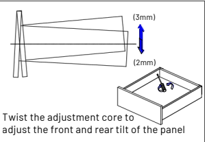
Drawer front assembly
