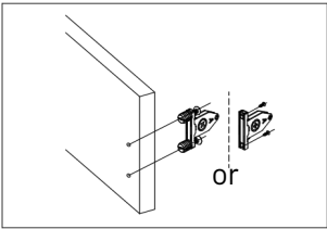
Up & down (height) adjustment :±2mm
